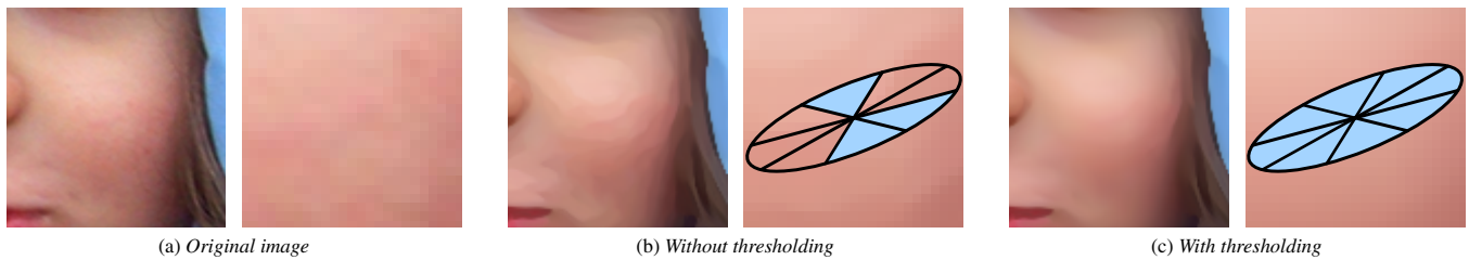
Figure 9: Comparison of weight computation with and without thresholding.
