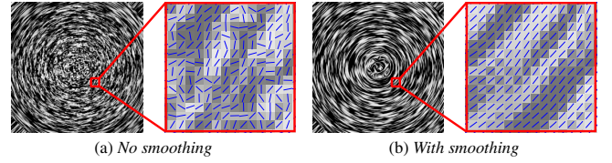
Figure 3: Visualization of the minor eigenvector of the structure tensor for a test ring pattern corrupted with Gaussian noise of variance v = 0.02 .
