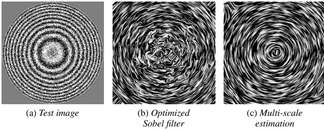
Figure 5: Visualization of the minor eigenvector field of the smoothed structure tensor ( \rho = 2 ) for a test ring pattern corrupted by Gaussian noise of variance v = 0.25 .
