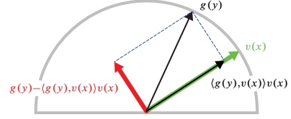
Figure 4: Deviation of a gradient g(y) := \nabla(y) from a given direction v(x) . The term \langle g(y), v(x) \rangle v(x) is the projection of g(y) onto v(x) .
