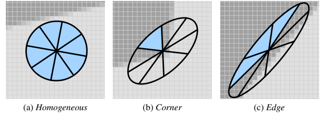
Figure 8: The anisotropic Kuwahara filter uses weighting functions defined over an ellipse, whose shape is based on the local orientation and anisotropy. The filter response is defined as a weighted sum of the local averages, where more weight is given to averages with low standard deviation.
