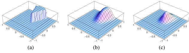
Figure 7: Construction of the weighting functions of the anisotropic Kuwahara filter: (a) Characteristic function \chi_0 . (b) \chi_0 \star G_\rho . (c) K_0 = (\chi_0 \star G_\rho) \cdot G_\sigma .
