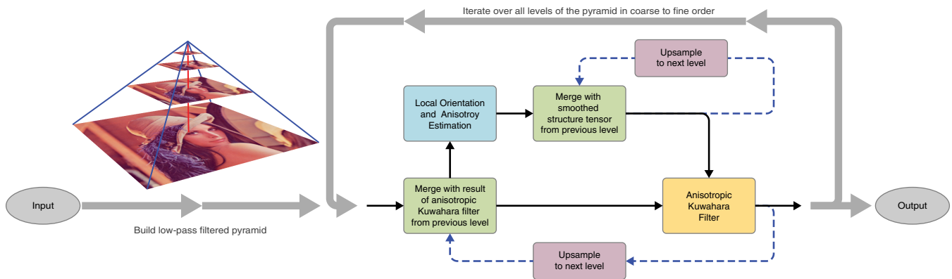
Figure 2: Schematic overview of the proposed technique.
