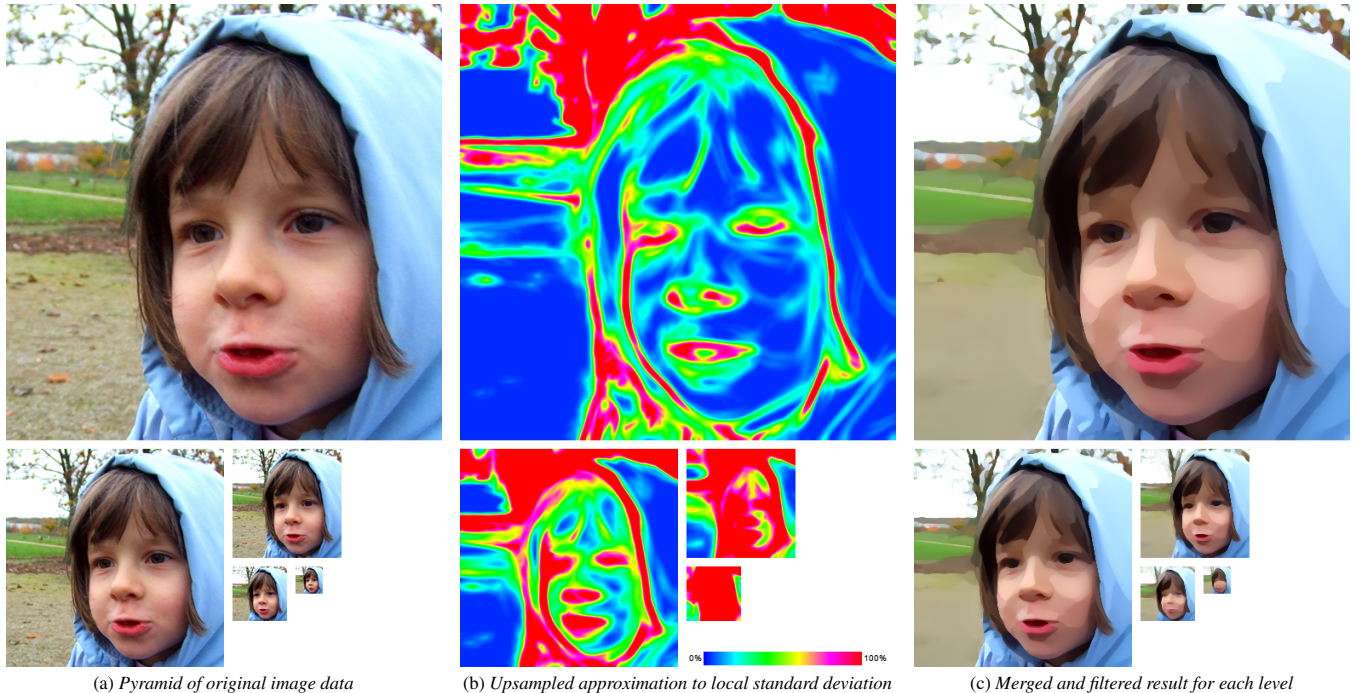
Figure 10: Original image, approximation to standard deviation and output of the anisotropic Kuwahara filter for the different pyramid levels.
